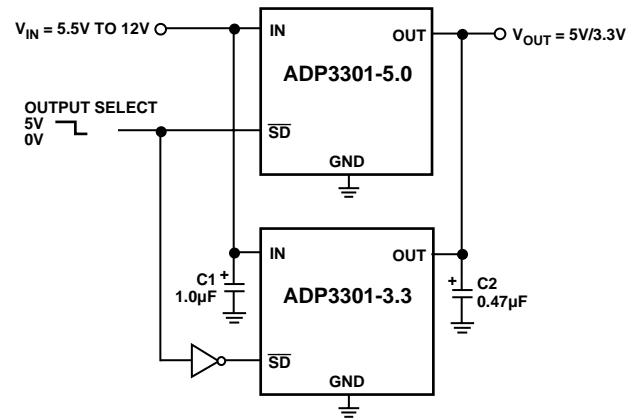
Figure 21. Crossover Switch
